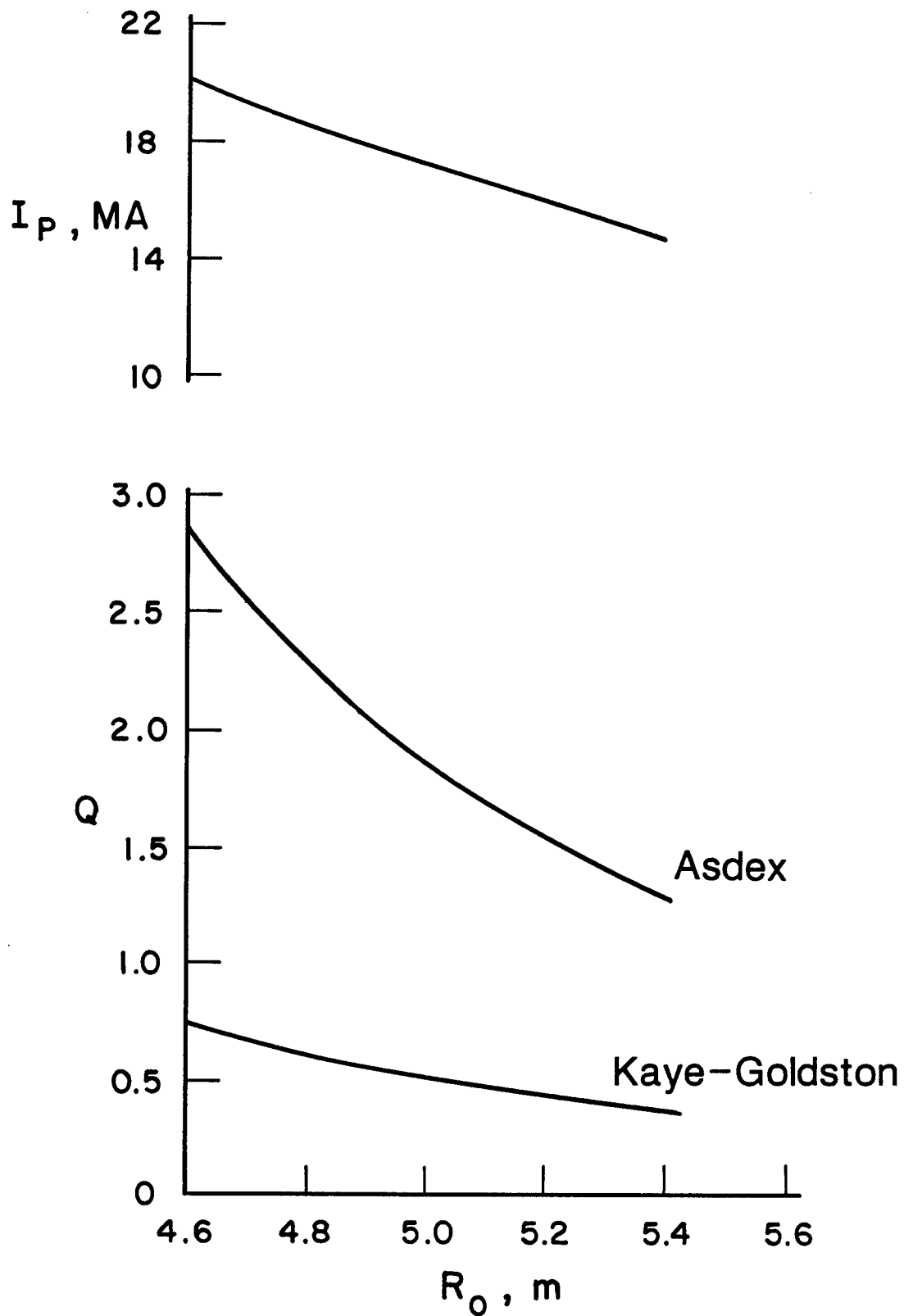
Fig. 3.3-5. Q and plasma current versus major radius; a = 1.69 m, B_c = 10.4 T, K = 2.17 , \langle T_1 \rangle = 37 keV.
