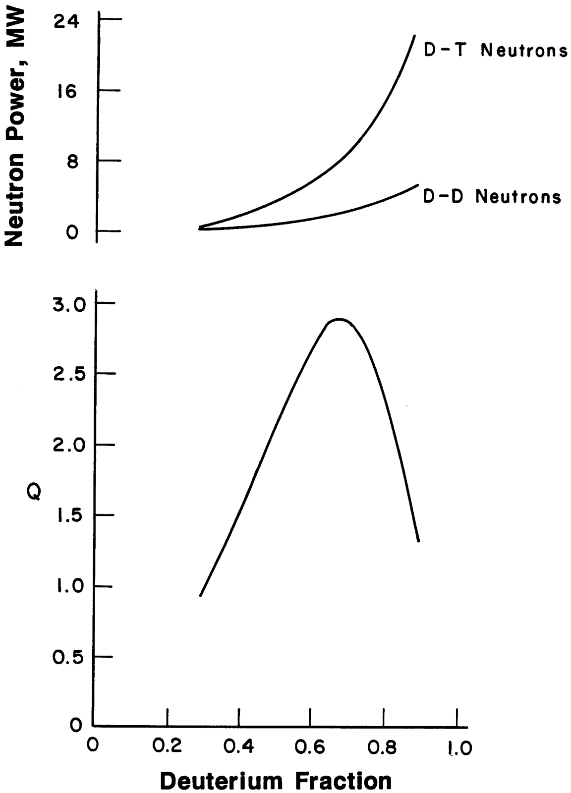
Fig. 3.3-6. Effect of changing fuel mixture on the energy multiplication, Q , and neutron power. R = 4.61 m, B_c = 10.4 T, \langle T_i \rangle = 37 keV, ASDEX H-mode scaling.
