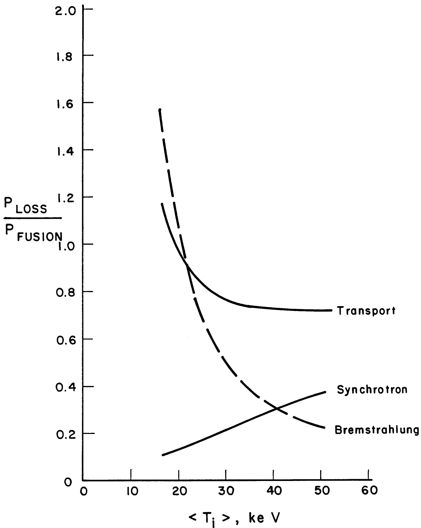
Fig. 3.3-7. Distribution of power loss versus average ion temperature. R = 4.61 m, B_c = 10.4 T, f_d = .65 , ASDEX H-mode scaling.
