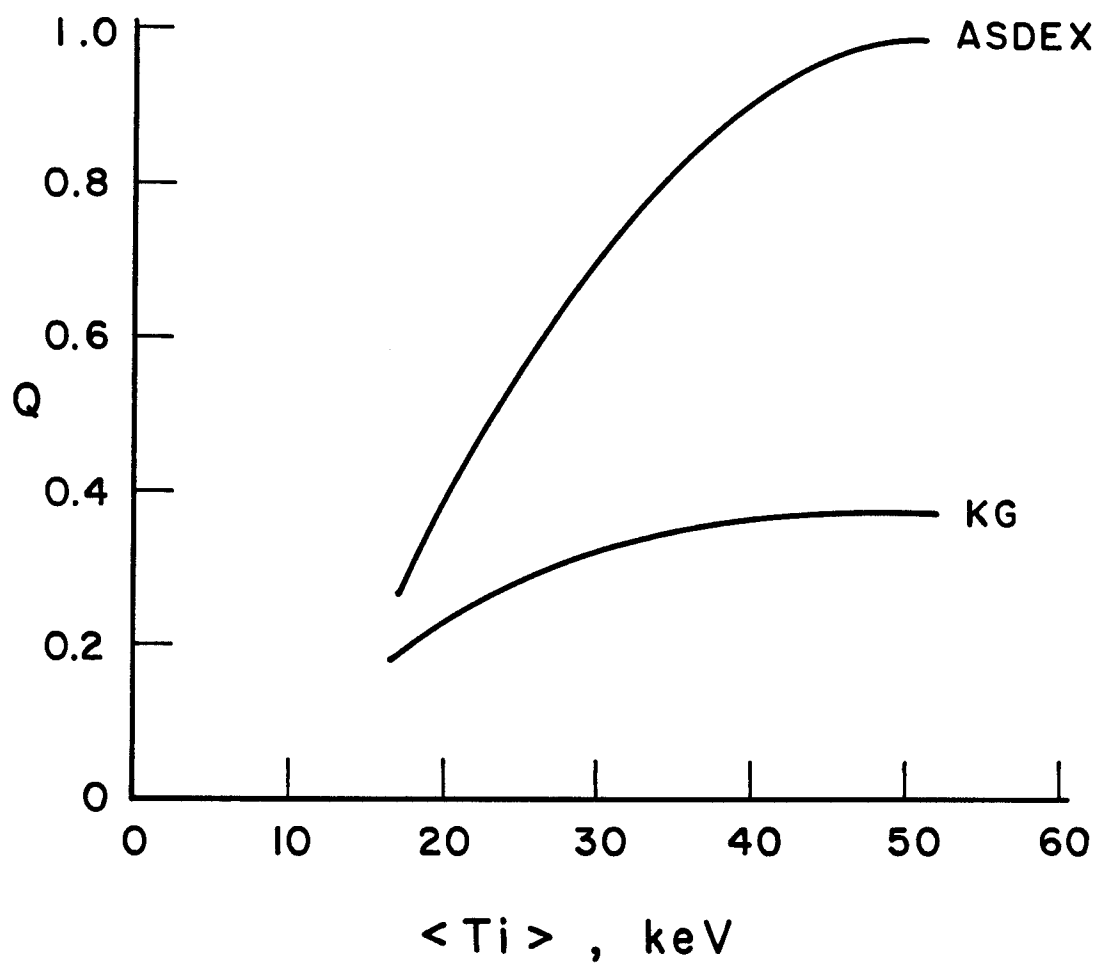
Fig. 3.3-1. Energy multiplication, Q , versus average ion temperature for D- ^3\text{He} operation in NET-DT for both ASDEX H-mode and Kaye-Goldston energy confinement scaling.
