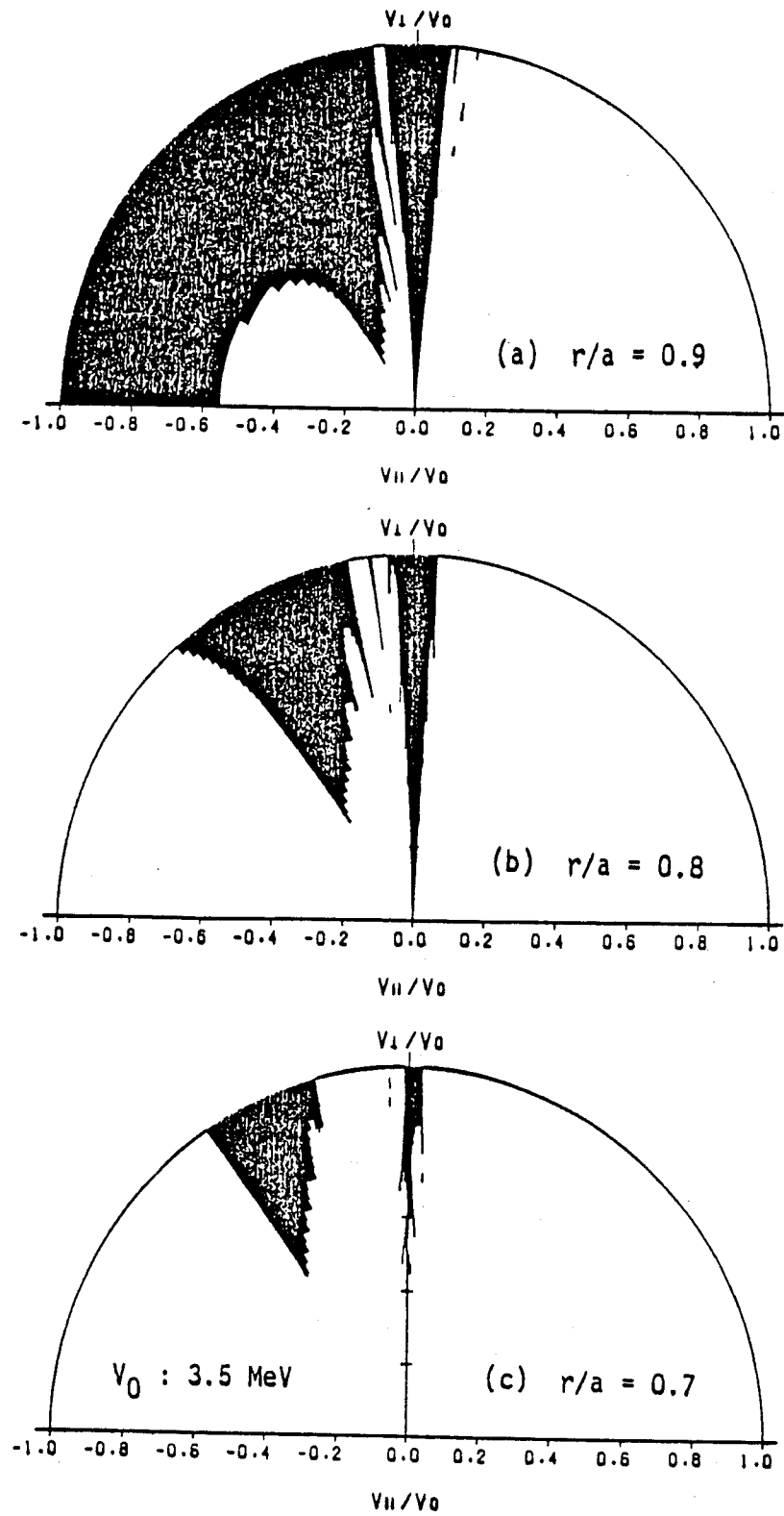
Fig. 5.3-4. Prompt (first-orbit) loss and ripple loss regions for INTOR with \delta_0 = 0.75\% from Tani et al. (7)
