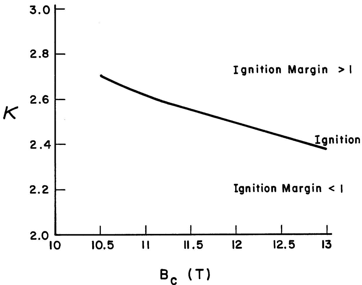
Fig. 3.3-10. The elongation required to achieve ignition versus toroidal magnetic field at the magnet. Points above the curve have ignition margin above 1; points below are subignited. R = 4.61 m, a = 1.69 m, \langle T_i \rangle = 37 keV, ASDEX H-mode scaling.
