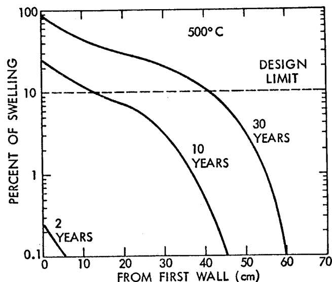
Fig. 8. Anticipated maximum swelling for 20% cold-worked Type-316 stainless steel in UWMAK-I blanket.
