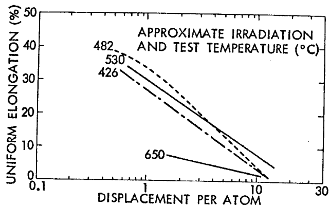
Fig. 5. Effect of displacement damage on the uniform ductility of solution-treated Type-316 stainless steel (Refs. 20 through 26).
