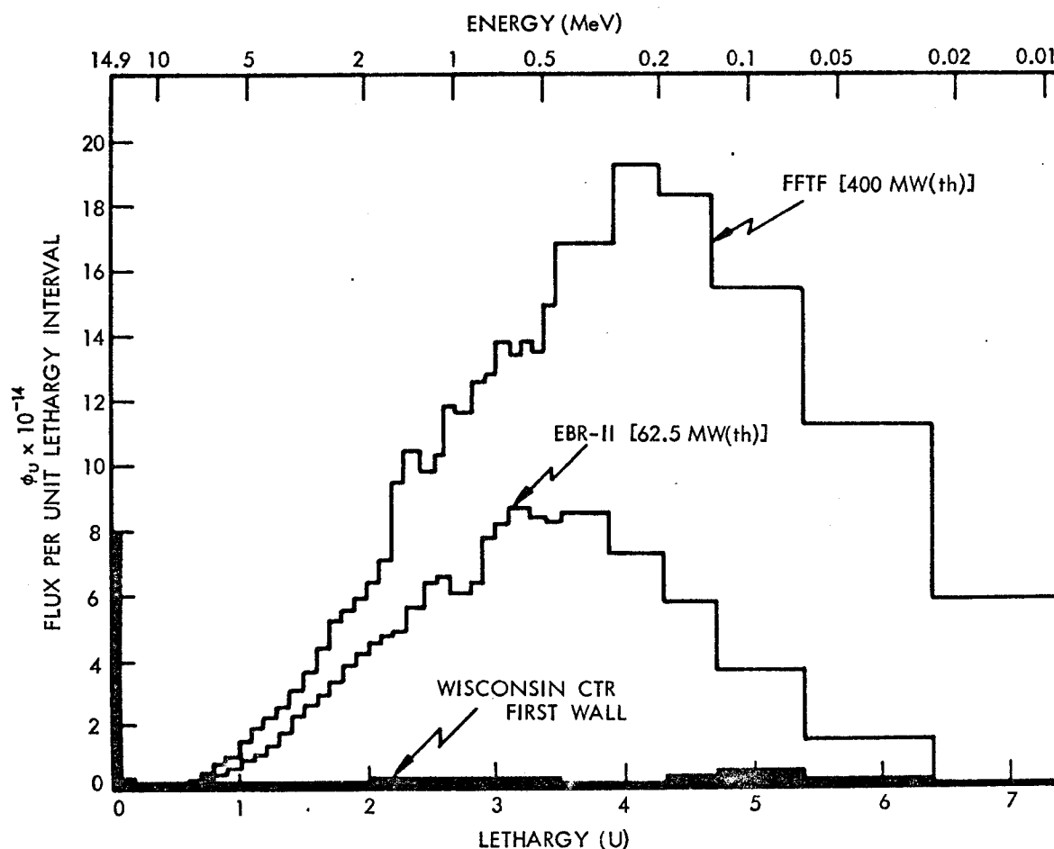
Fig. 3. Comparison of calculated neutron spectra for UWMAK-I [5000-MW(th)] fusion reactor to EBR-II and FFTF fission reactors.
