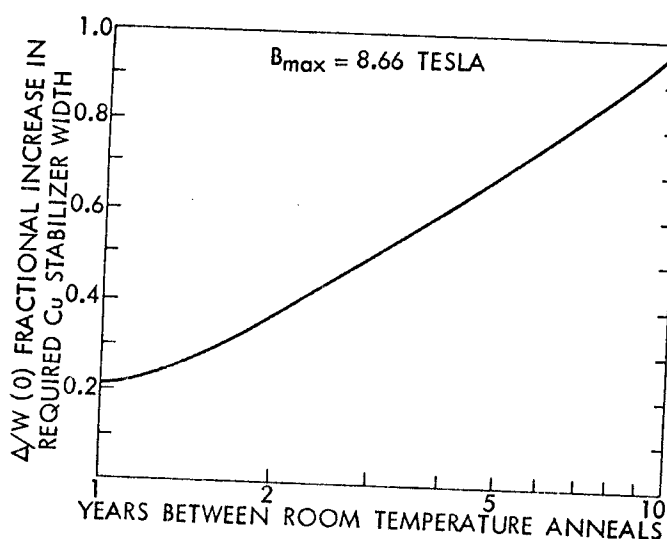
Fig. 12. The effect of periodic room-temperature anneals on the required thickness increase in copper stabilizer in UWMAK-I magnets.
