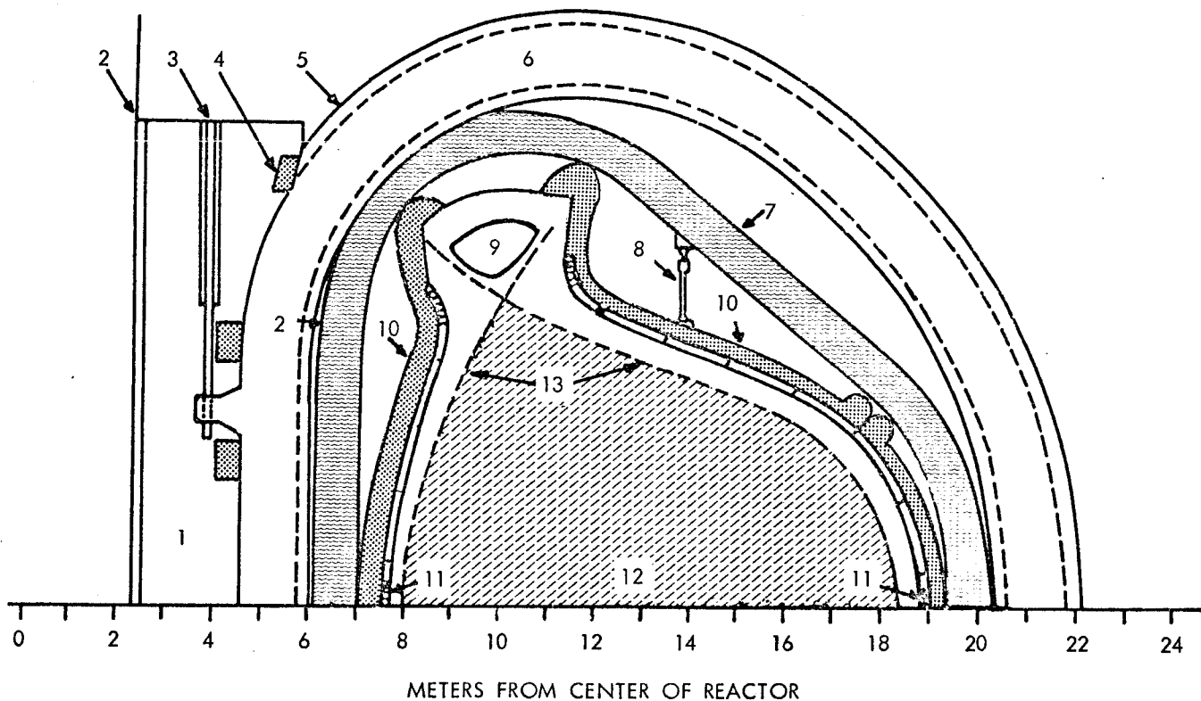
Fig. 1. Schematic view of UWMAK-I fusion reactor:
