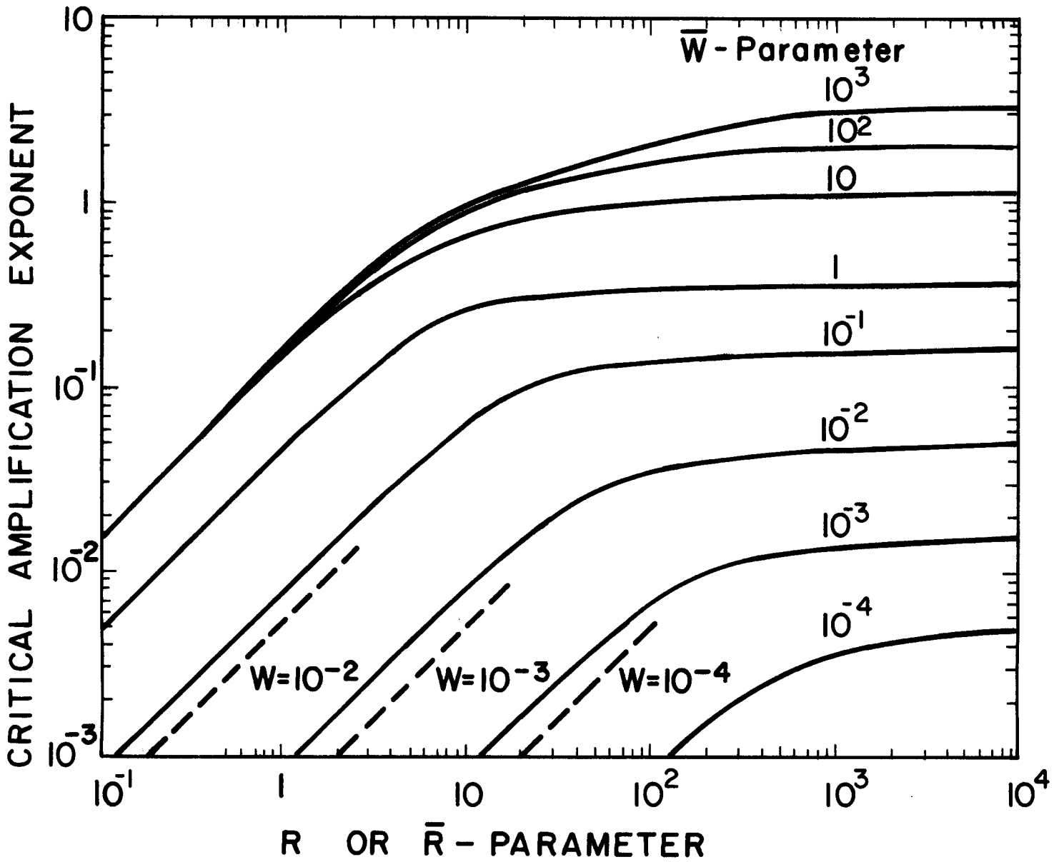
Figure 2 Variation of the critical amplification exponent with surface Reynolds number.
