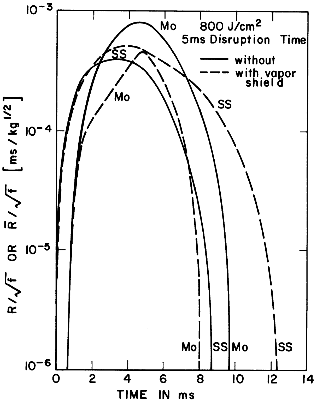
Figure 3 Time variation of R/\sqrt{f} for 800 J/cm 2 and 5 ms disruption time.
