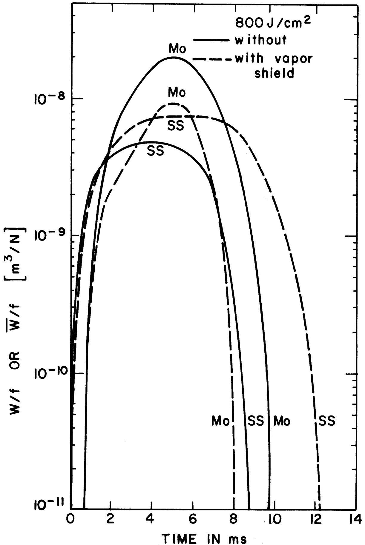
Figure 4 Time variation of W/f for 800 J/cm 2 and 5 ms disruption time.
