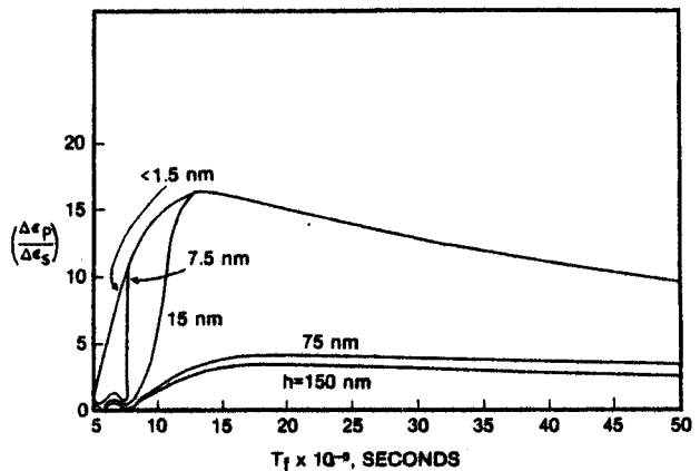
Fig. 1. The enhancement factor for nickel at 200°C as a function of the total cycle time for a given barrier height, h . T = 5000\text{s} , \rho_d = 2 \times 10^{13} \text{ m}^{-2} , P = 10^{-6} dpa/s, and all other material parameters are taken from ref. [1].
