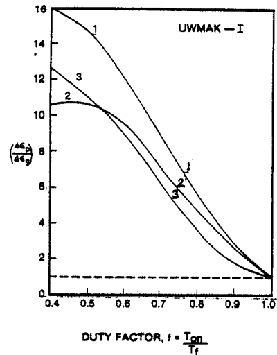
Fig. 3. The enhancement factor for UWMAK-I as a function of the duty factor, using different damage rates. Curve 1: dose-equivalent averaged damage rate; curve 2: equal instantaneous damage rates, dose not conserved; curve 3: equal instantaneous damage rates, dose conserved; All other conditions are the same as in Fig. 2.
