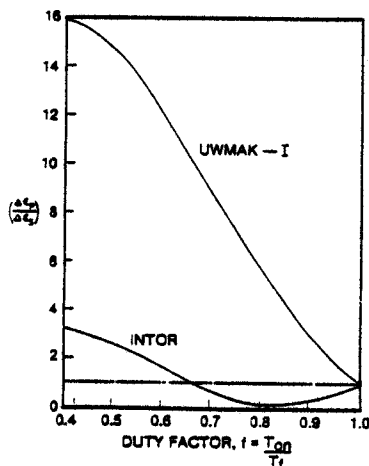
Fig. 2. The enhancement factor for UWMAK-I and INTOR as a function of the duty factor. Stain less steel at T=3000^{\circ}\text{C} , P=10^{-6} dpa/s, \rho_d=10^{12}/\text{m}^2 for UWMAK-I and \rho_d=10^{14}/\text{m}^2 for INTOR. All other material parameters are taken from ref [1].
