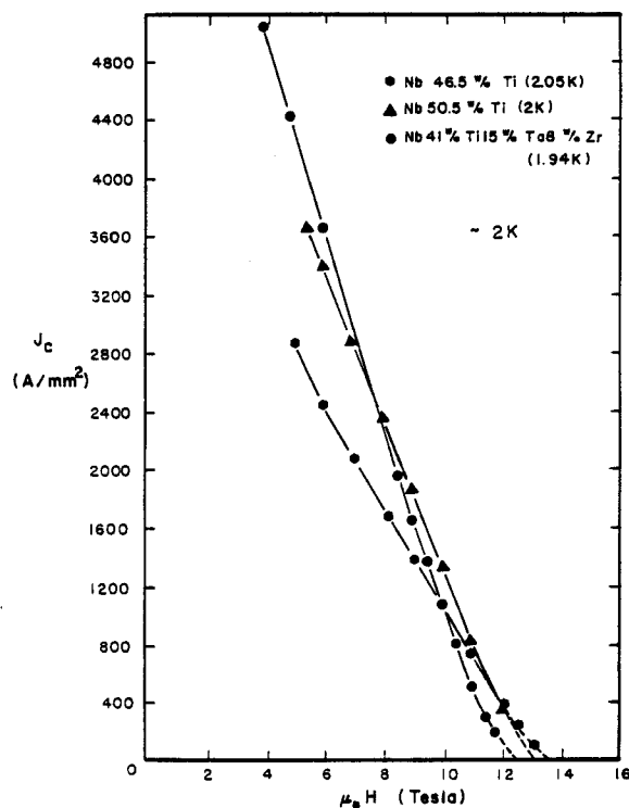
Fig. 13. Current densities of commercial composites at about 2K[9,26].
