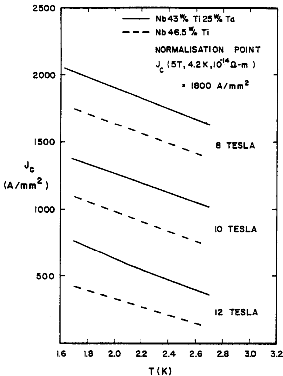
Fig. 17. Comparison of the predicted J_c values at 8, 10 and 12 Tesla for Nb 46.5w/o Ti and Nb 43w/o Ti 25w/o Ta composites (Courtesy D.G. Hawsworth).
