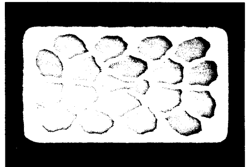
Fig. 19. Compacted monolith conductor for EBT made of 19 Brookhaven Isabelle design strands (Courtesy of S.O. Hong).
