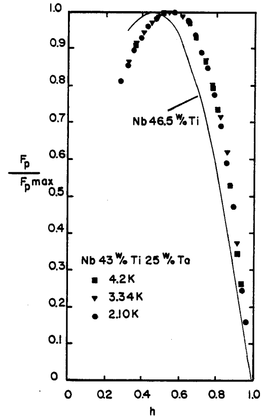
Fig. 18. Reduced pinning force curves for Nb 46.5w/o Ti and Nb 43w/o Ti 25w/o Ta multifilamentary composites[28].
