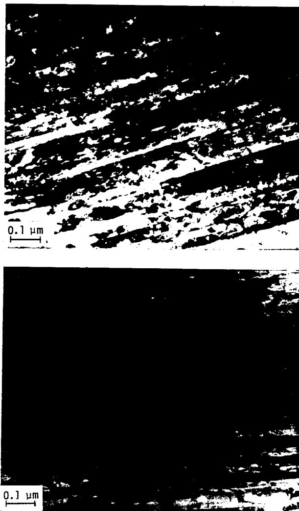
Fig. 14. Transmission electron micrographs of Fermilab composites at final size. The upper has received no heat treatment, the lower 160 hours at 375°C[21,39]. See text for details.
