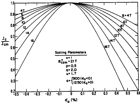
Fig. 28. Relative critical-current density J_c/J_{c_m} as a function of intrinsic strain \epsilon_0 (= \epsilon - \epsilon_m) for different magnetic fields evaluated using Eq. (3) and the typical set of scaling parameters indicated in the figure [79].
