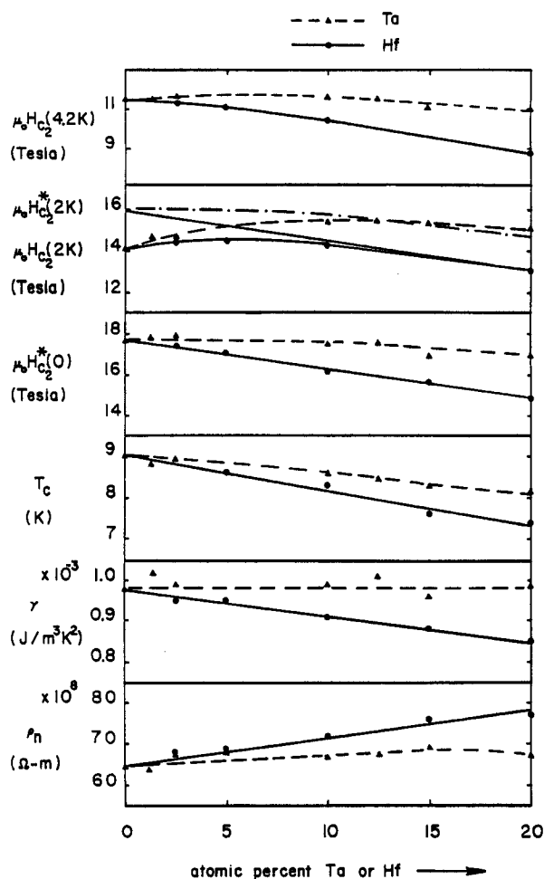
Fig. 6. The variation of \rho_n , \gamma , T_c , and the theoretical GLAG and experimental upper critical fields, \mu_0 H_{c2}^* and \mu_0 H_{c2} for Nb-Ti-Ta and Nb-Ti-Hf alloys of constant electron to atom ratio (4.35) [9,28].
