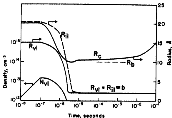
Fig. 5. Microstructure components for a single irradiation pulse in Zone 2.
