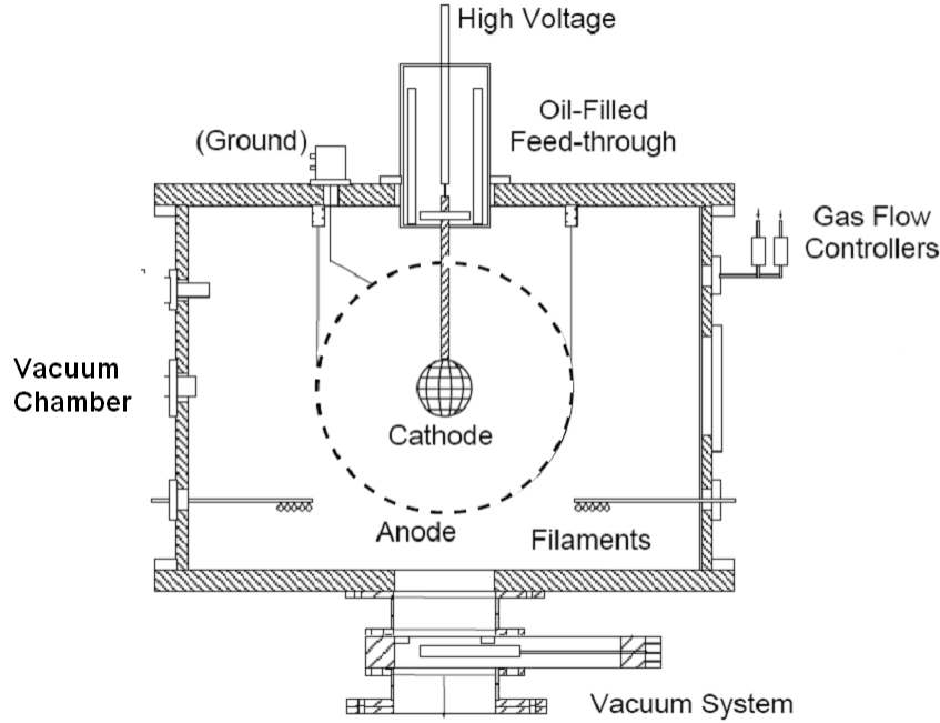
Figure 1. Schematic of the University of Wisconsin IEC device.
