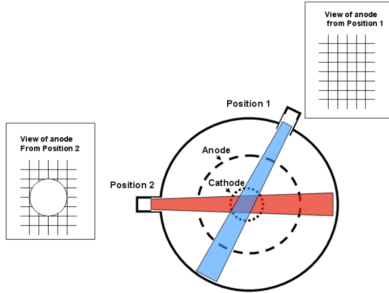
Figure 9. Shows the two positions and corresponding lines of site on which the Faraday trap diagnostic was oriented.
