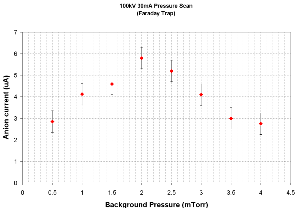
Figure 11. The pressure scan illustrates how the deuterium anion current detected in the Faraday trap has a maximum for 2 mTorr of background gas. This is due to increasing neutral pressure resulting increasing anion creation up to 2 mTorr with further increases in background pressure resulting in attenuation of the anion flux to the detector.
