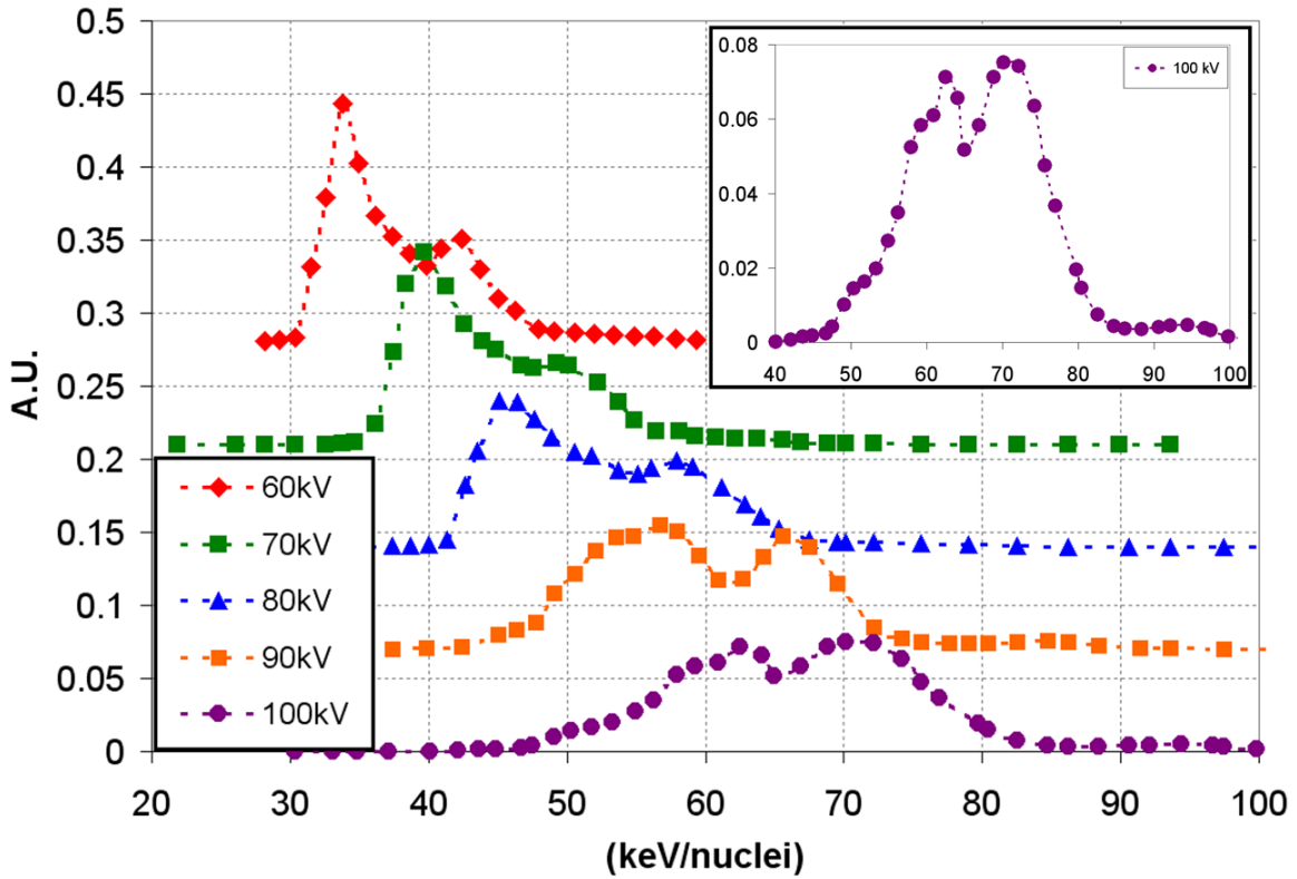
Figure 4. The deuterium anion spectra are plotted for several cathode voltages offset by 0.07a.u. for every 10 kV. These show a clear hardening of the spectra with increasing cathode voltage. In addition the spectra change from being dominated by D_3^+/D^- at lower voltages (60 kV – 80 kV) charge transfer ions to being dominated by D^+/D^- charge transfer ions at higher voltages (90 kV-100 kV). Error bars from counting statistics are negligible on the scale shown. Detail of 100 kV data set shown in upper right.
