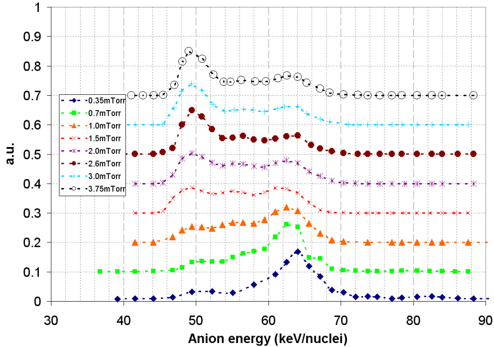
Figure 7. Pressure scan with cathode voltage and cathode current held constant at 90 kV, and 30 mA respectively. Note that the ratio of the D_3^+ / D^+ peak to the D^+ / D^+ peak changes dramatically over the scan. Each successive data set is offset by 0.1 a.u.
