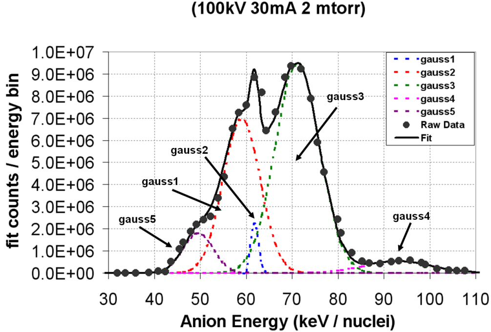
Figure 5. Detailed view of the 100 kV, 30 mA, 2 mTorr, data set. It shows the 5 Gaussian least squares fit used to accurately replicate the structure from the data set. The fits “gauss1”, “gauss2” and “gauss3” account for deuterium anions produced through D_3^+/D^- , D_2^+/D^- and D^+/D^- charge transfer reactions respectively. The “gauss 4” fit is accounted for by D^- formed at the cathode via thermal electron attachment to background neutral gas. The “gauss5” fit is accounted for by metastable D_2^- formed via thermal electron attachment at the cathode.
