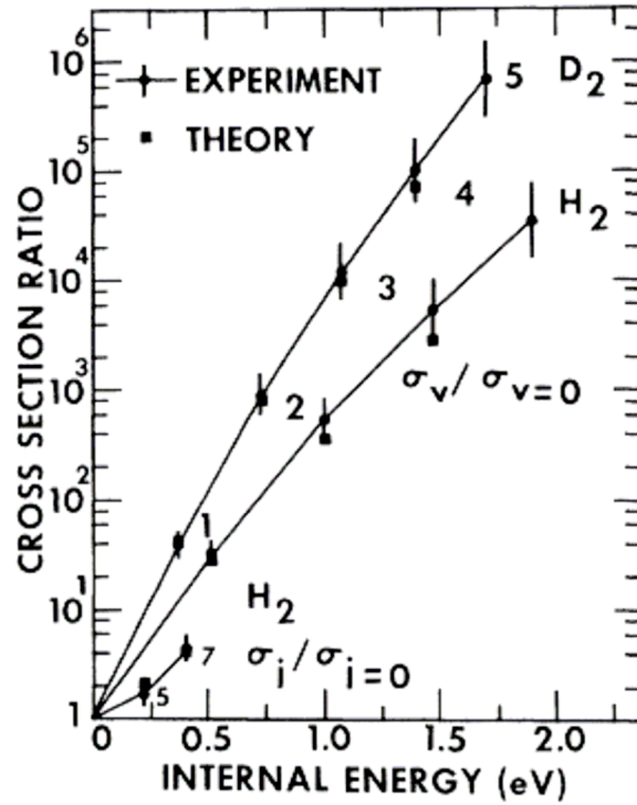
Figure 2. The above data from Allen and Wong indicates cross section for dissociative thermal electron attachment in D_2 to vary between 8 \times 10^{-24} \text{ cm}^2 and \sim 6 \times 10^{-18} \text{ cm}^2 depending on the internal energy of the molecule. 16
