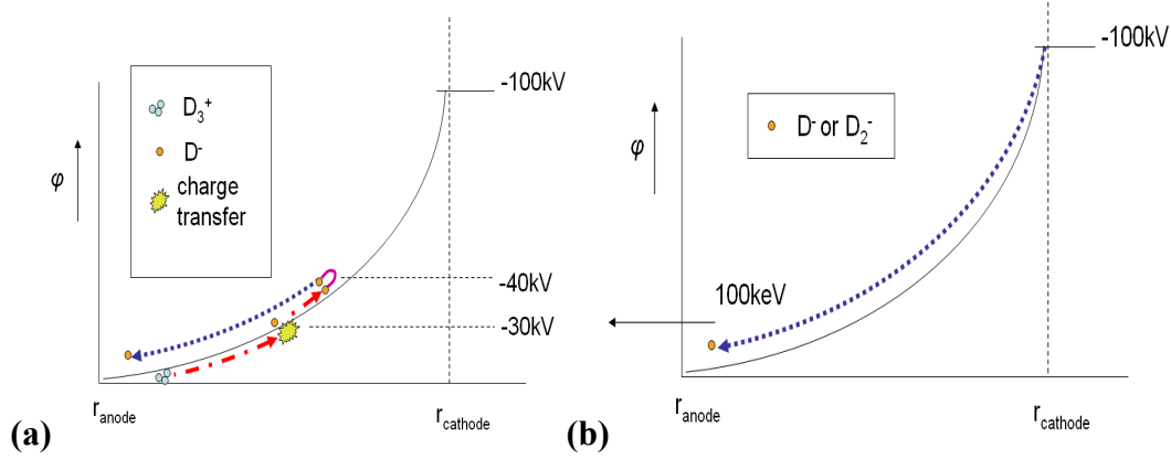
Figure 6. Illustrates examples of the resulting deuterium anion energies from (a) charge transfer reactions in the intergrid region of the UW IEC device, and (b) thermal electron attachment near the cathode of the UW IEC device. Note that the anions resulting from the thermal electron attachment will have 100 keV/anion so a D^- ion will have 100 keV and a D_2^- ion will have 50 keV/nuclei with the cathode at 100 kV.
