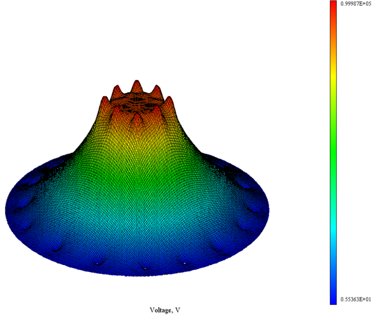
Figure 10. The schematic above shows a 2-D cylindrical representation of the potential profiles between an IEC cathode and anode with -100 kV on the cathode. The perturbations near the cathode in the 2-D representation are ~5-10 kV. This will be reduced in a 3-D geometry but still substantial for cold anions and electrons born near the cathode.
