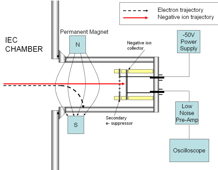
Figure 8. Shows a schematic of the Faraday trap diagnostic illustrating differing negative ion and electron trajectories. The negative ion collector plate and secondary electron suppressor grid are isolated from the chamber and each other by ceramic standoffs. The magnetic field is 100 gauss, and its orientation has been rotated by 90° in the image above so as to show the spatial extent of the magnetic field.
