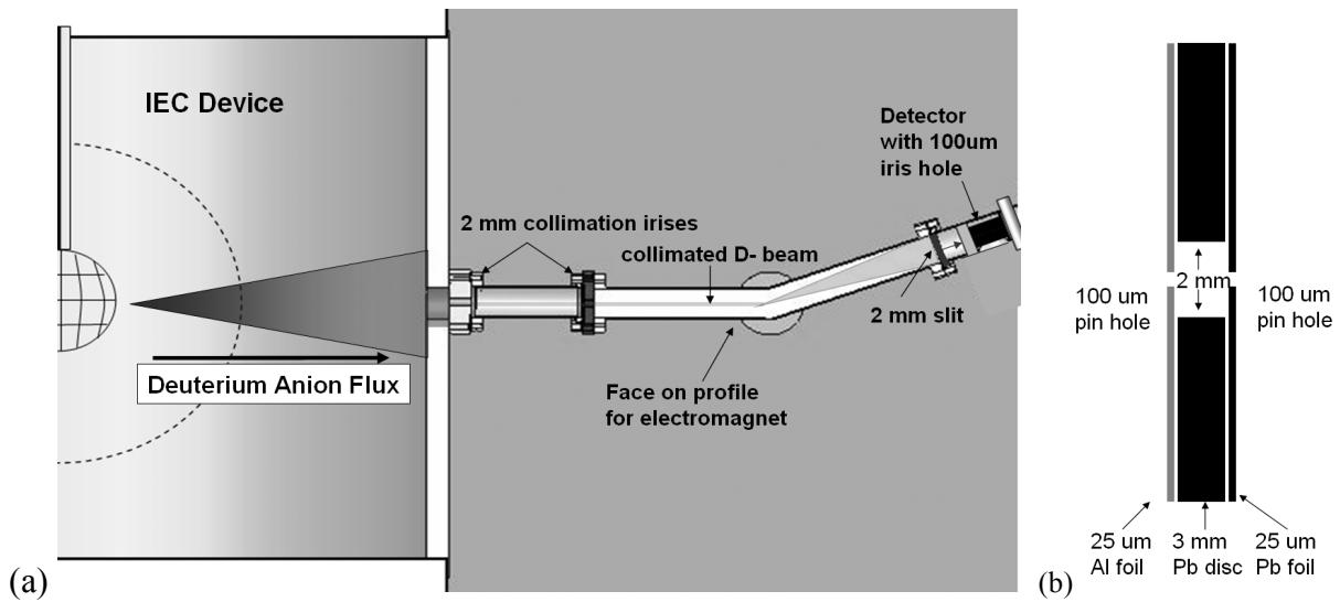
Figure 3. (a) Shows schematic of the magnetic deflection energy analyzer. (b) Shows a closeup of the construction of the 100 \mu\text{m} iris hole (not to scale) used to both limit particle flux to the detector and narrow the energy resolution of the diagnostic. The 100 \mu\text{m} iris sits on the face of the detector.
