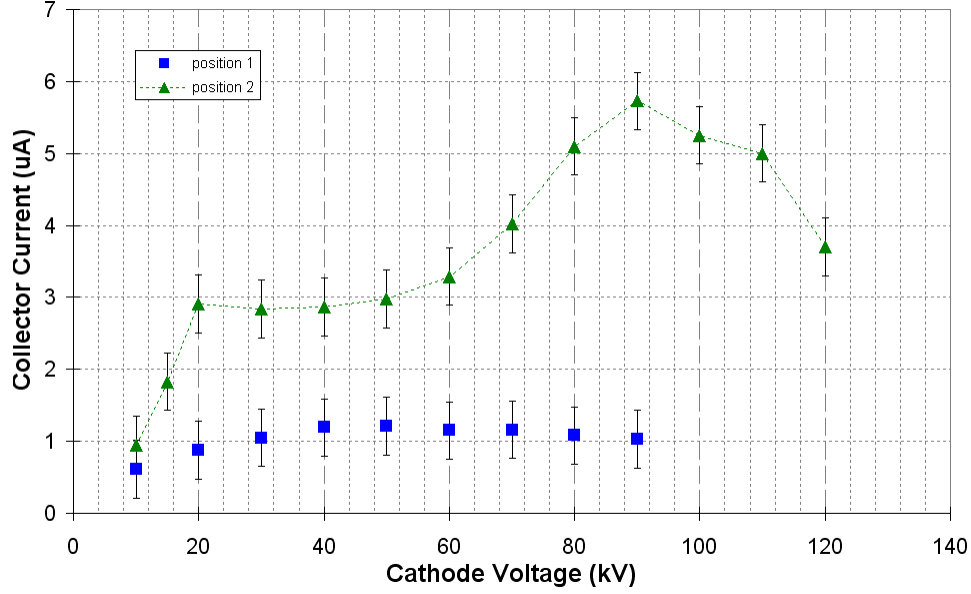
Figure 12. Position 1 shows a sub-linear dependence of collector current on voltage, with a maximum between 40-50 kV. Position 2 shows a greater than linear dependence of collector current on voltage with a maximum at 90 kV. At both positions the cathode current was 30 mA and the background pressure was 2 mTorr.
