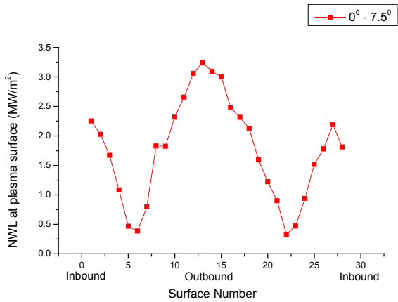
Fig. 9. The neutron wall load profile at 0 – 7.5 degree toroidal section
