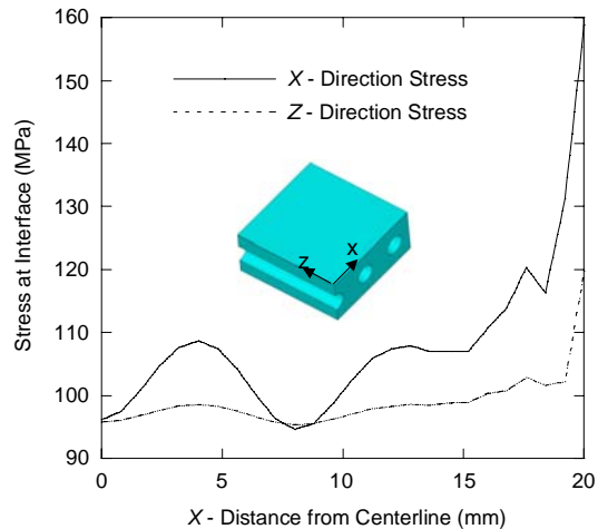
Fig. 11. Thermal stresses in the armor at the steel interface for the cooled IR test specimens
