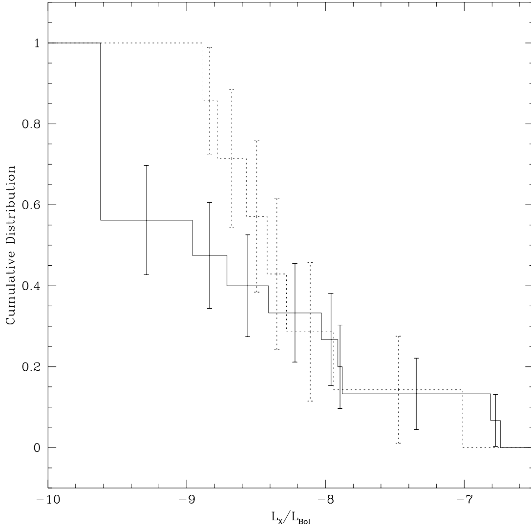
Fig. 4.— Cumulative L_X/L_{\text{Bol}} distributions of the Be stars (dotted line) and non-Be B V stars with spectral type B1.5 or later (solid line).
