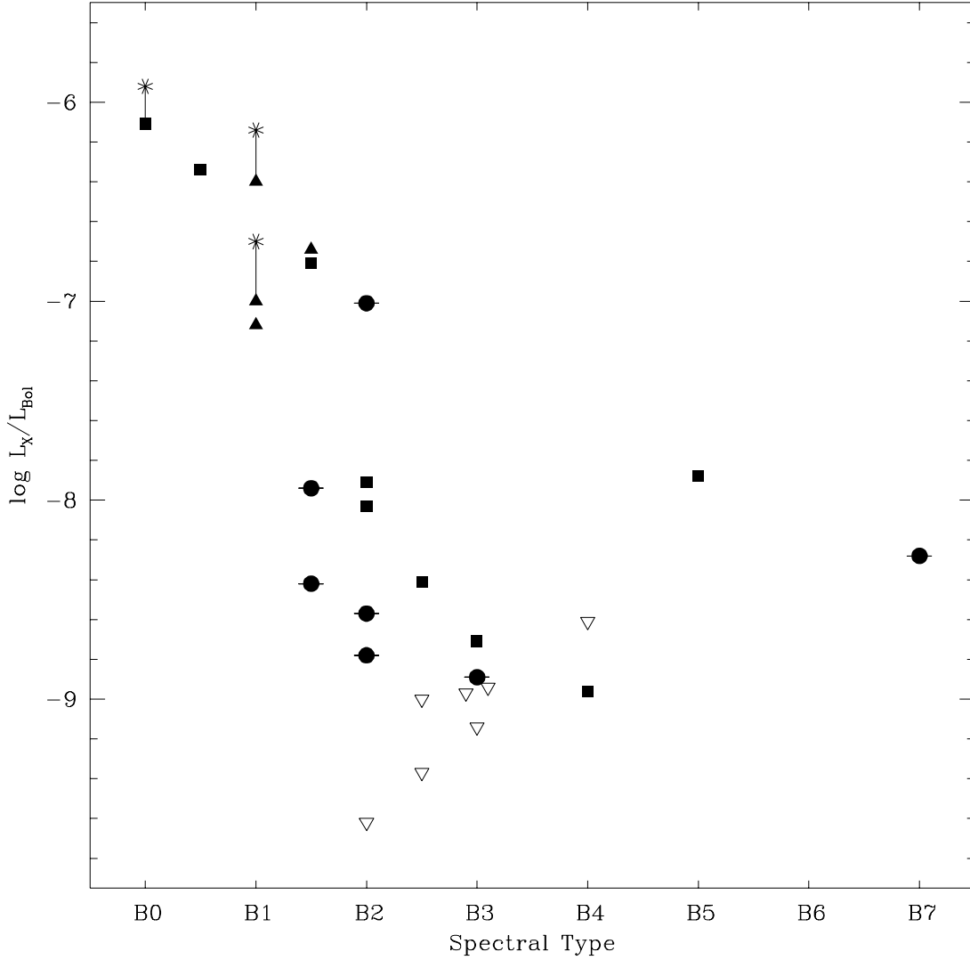
Fig. 2.— We show the ratio L_X/L_{\text{Bol}} for each of the 20 program stars which were detected above the 3\sigma level. For three stars, \tau Sco, \beta Cen, and \xi^1 CMa, we indicate the total generated luminosities with asterisks, which are connected to the points representing the emergent x-ray luminosities with a line. Upper limits ( 3\sigma ) for seven stars are indicated with open triangles. Be stars are indicated by circles with lines and \beta Cephei variables by filled triangles.
