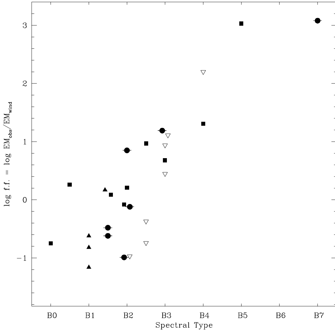
Fig. 3.— We show the wind filling factors for each of the 20 program stars which were detected above the 3\sigma level. Upper limits for seven additional stars are indicated with open triangles. Be stars are indicated by circles with lines and \beta Cephei variables by filled triangles.
