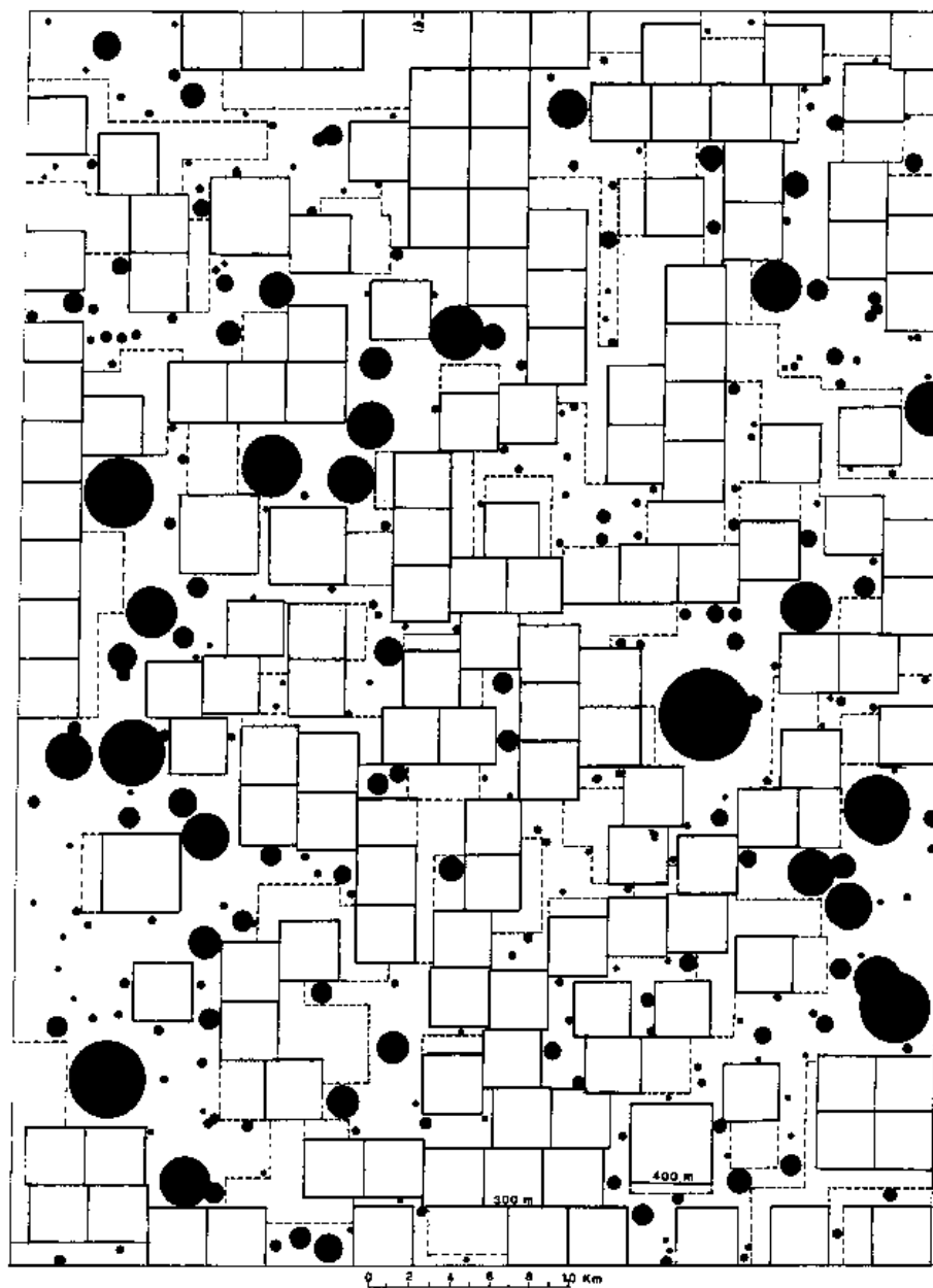
Figure 7. Reduced overlay of original of Figure 5. Craters 23.4 m or more in diameter (including ejecta halos where observed or inferred) shown by solid black circles. Movable area plotted largely in terms of 300-meter square blocks (bounded by solid lines) and extensions (bounded by dashed lines).
