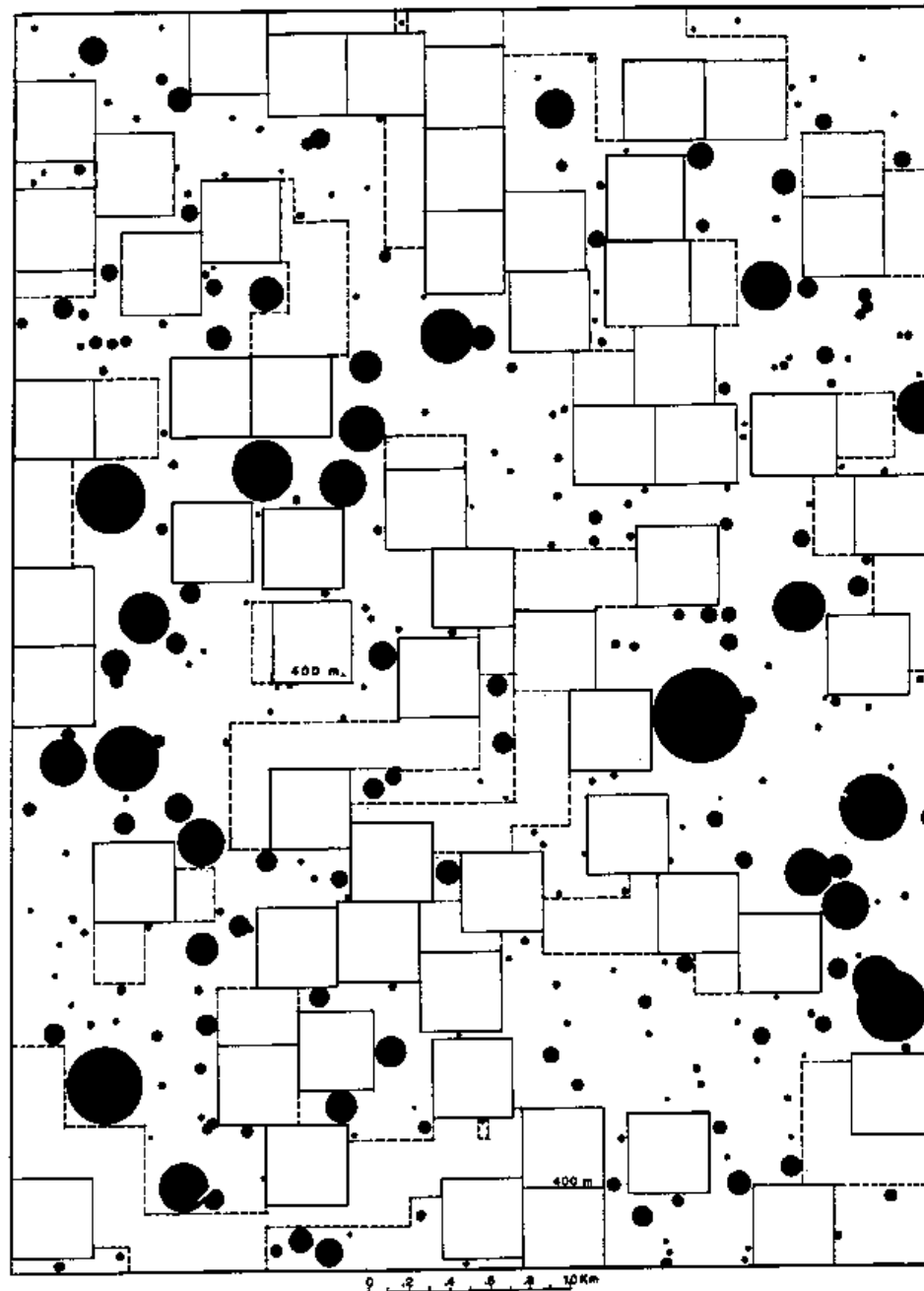
Figure 6. Reduced overlay of original of Figure 5. Craters 23.4 m or more in diameter (including ejecta halos where observed or inferred) shown by solid black circles. Minable area plotted in terms of 400-meter square blocks (bounded by solid lines) and extensions (bounded by dashed lines).
