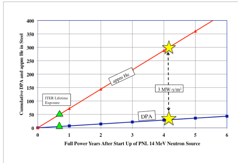
Fig. 5. The PNL 14 MeV neutron facility can simulate 3 MW-y/m 2 in ~4 FPY.
