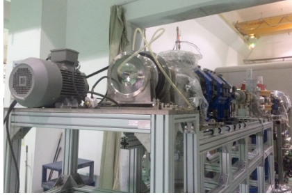
Fig. 1-a. Steady beam line.
