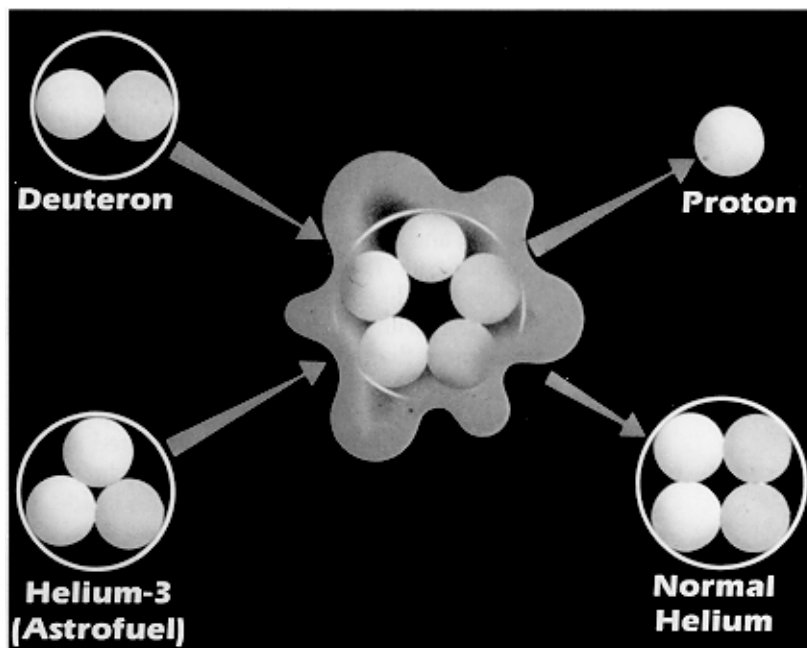
Figure 3. The Astrofuel fusion reaction, which releases 18.4 MeV of energy per event.
