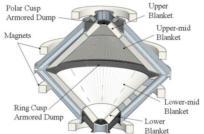
Fig. 1. Example chamber configuration with magnetic diversion.
