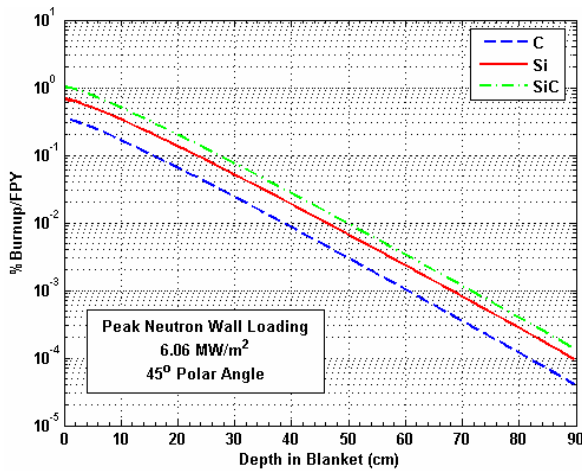
Fig. 4. Radial variation of burnup rate in the SiC.
