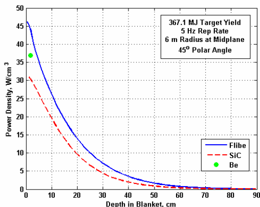
Fig. 3. Nuclear heating at 45^\circ polar angle.
