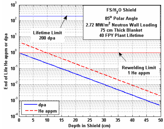
Fig. 6. Radial variation of dpa and He in F82H shield.
