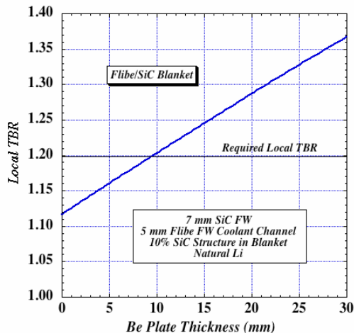
Fig. 2. Impact of Be insert thickness on TBR.
