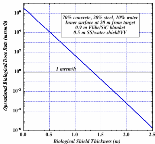
Fig. 7. Biological shield requirement.
