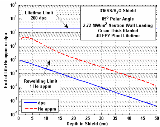
Fig. 5. Radial variation of dpa and He in 316SS shield.
