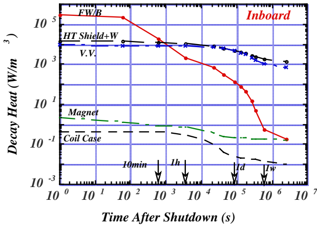
Figure 5. Inboard side decay heat.
