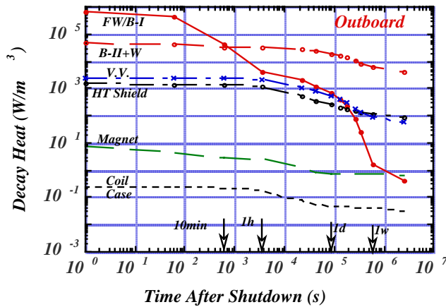
Figure 6. Outboard side decay heat.
