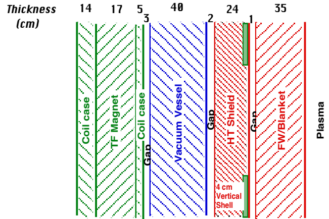
Figure 1. Inboard radial build.
