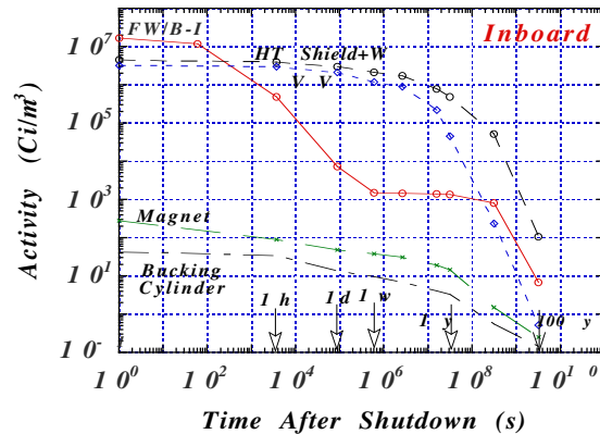
Figure 3. Inboard activity results.
