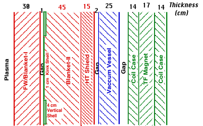
Figure 2. Outboard radial build.
