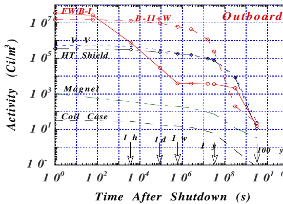
Figure 4. Outboard activity results.
